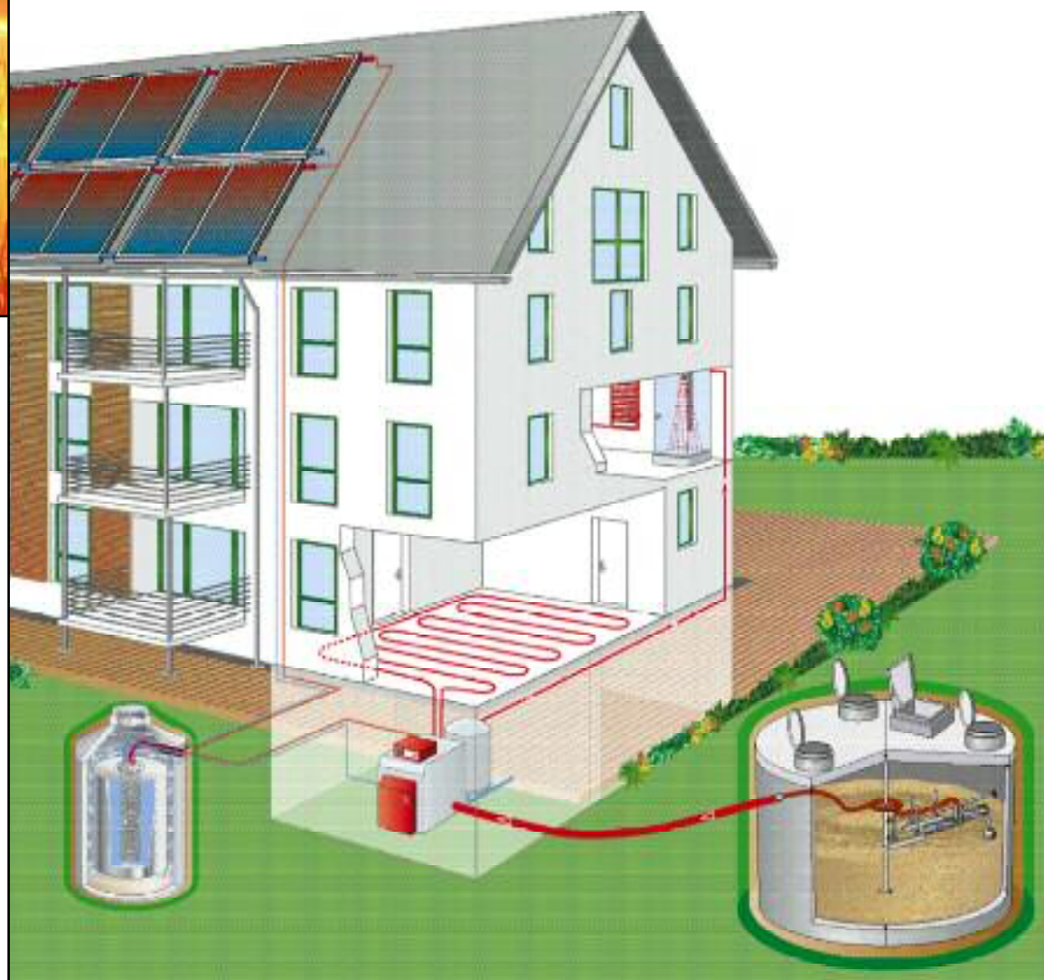
Mall-Pufferspeicher Solitherm
